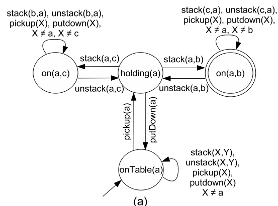
Figure 1: Automata of blocks world example.
